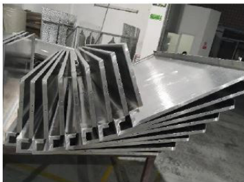
Fluoro-aluminum-zinc sheet bending
